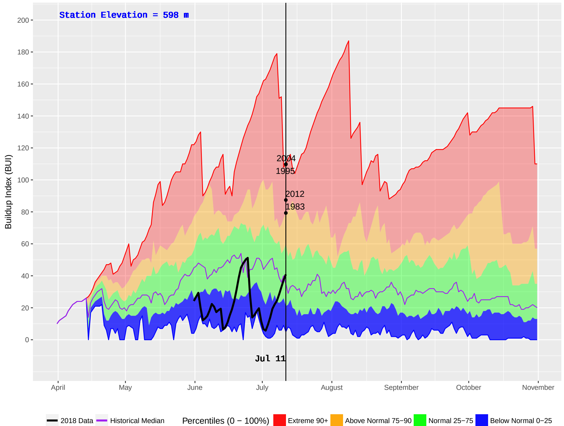
HELMUT (118) : Historical (1983–2016) and Current (2018) Noon Buildup Index (BUI)
