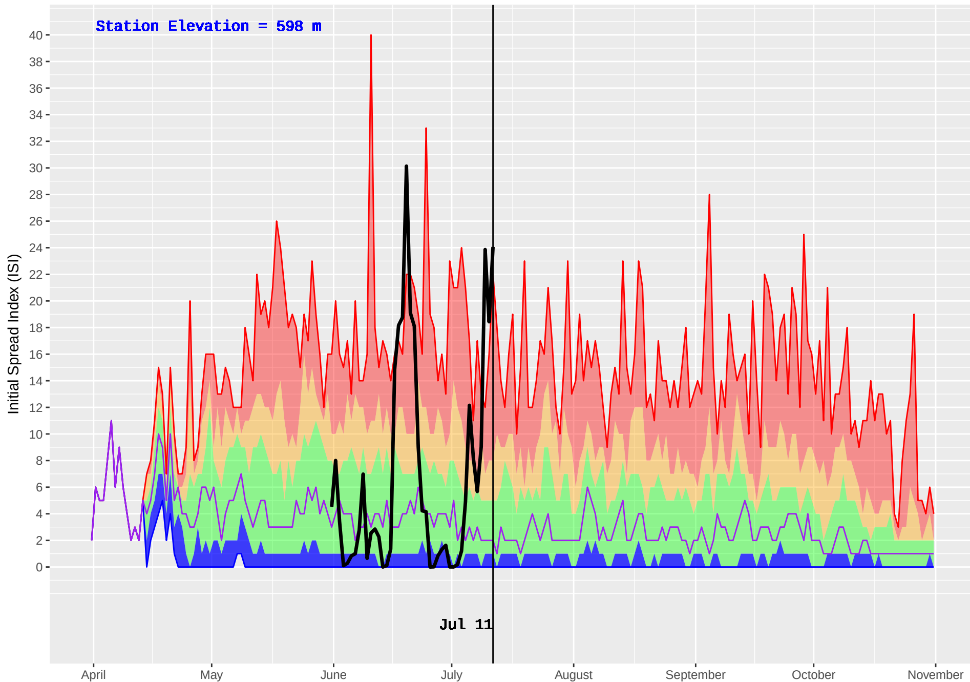
HELMUT (118) : Historical (1983–2016) and Current (2018) Noon Initial Spread Index (ISI)
